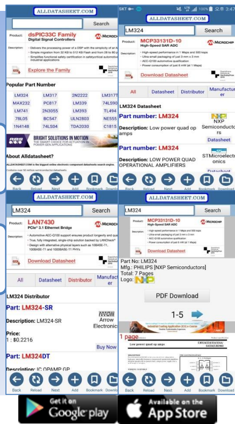
[Mobile application]
